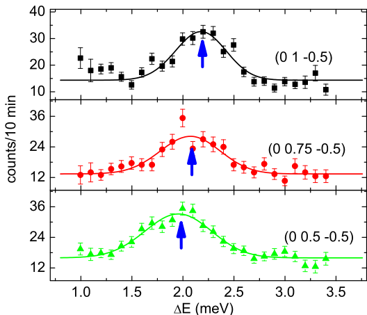
FIG. 5. Constant-Q scans along the zone boundary points ranging from (0\ 1\ -0.5) to (0\ 0.5\ -0.5) . The solid line are fits to a Gaussian. the data were collected on HB-1A.
