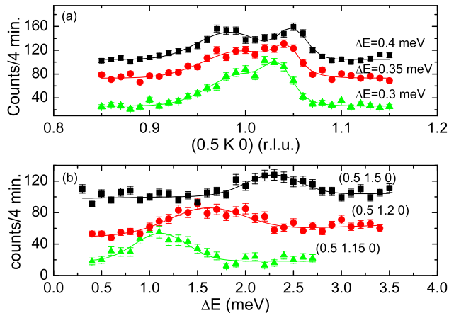
FIG. 3. (a) Constant- E scans along (0.5 K 0) collected in the HK0 scattering plane at T = 1.5 K by the CG-4C spectrometer. (b) Constant- Q scans collected in the HK0 scattering plane at T = 1.5 K by the CG-4C spectrometer. The solid lines in both panels are fits with Gaussians.
