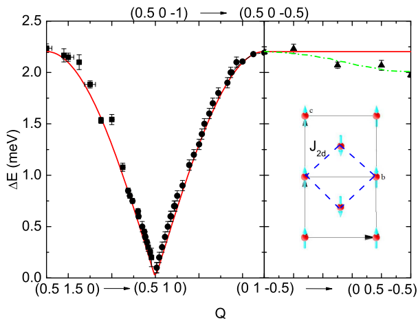
FIG. 6. Summary of the spin wave dispersion for \text{CuF}_2(\text{D}_2\text{O})_2(\text{d}_4\text{-pyz}) . The data were collected using CNCS (solid circles), CG-4C (solid squares) and HB-1A (solid triangles). The solid line represents the dispersion of Heisenberg linear spin wave theory with a nearest neighbor interaction. The dash-dotted line represents the results of series expansion to higher order. 15 The inset depicts the bc-plane. The dashed lines show the square lattice with a nearest neighbor exchange interaction.
