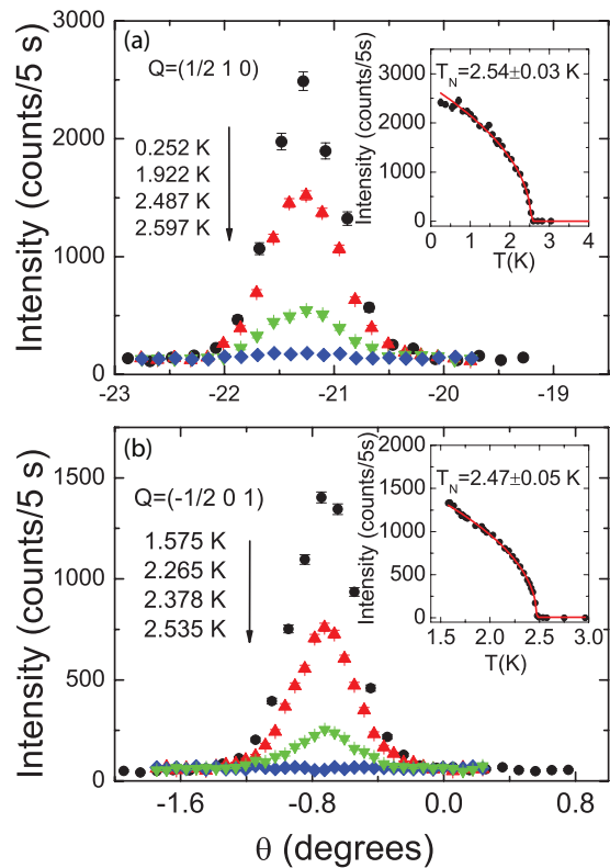
FIG. 1. (a) Temperature dependence of magnetic Bragg peaks (a): (0.5 \ 1 \ 0) and (b): (-0.5 \ 0 \ 1) for \text{CuF}_2(\text{D}_2\text{O})_2(\text{d}_4\text{-pyz}) . Insets display the temperature dependent peak intensity. Solid lines are guides to the eye. The data were collected on the HB-1 triple-axis instrument in HK0 and H0L scattering planes, respectively.
