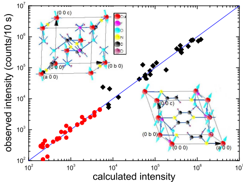
FIG. 2. The observed intensity plotted as a function of calculated intensity for \text{CuF}_2(\text{D}_2\text{O})_2(\text{d}_4\text{-pyz}) at T=0.25 K. Nuclear and magnetic reflections are denoted by diamonds and circles, respectively. The solid line is a guide to the eye. The data were collected on HB-1 in different scattering planes. The insets depict different views of the unit cell. The arrows on Cu atoms indicates the magnetic moment configuration. The 2d magnetic behavior of \text{CuF}_2(\text{D}_2\text{O})_2(\text{d}_4\text{-pyz}) originates in the bc plane.
