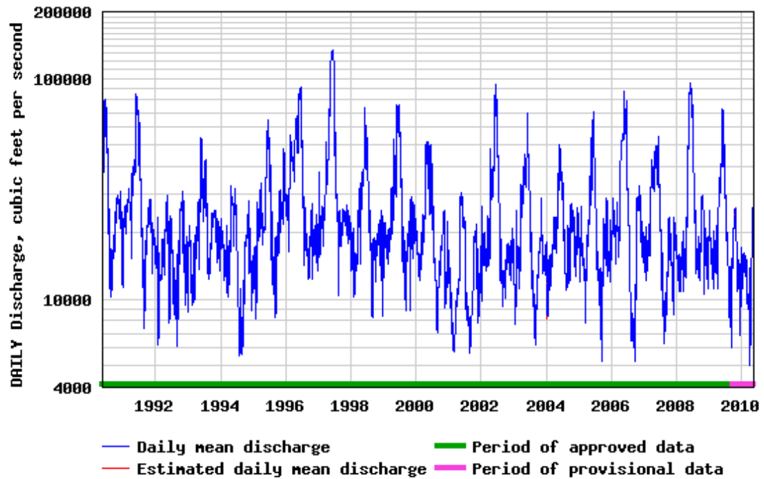
Figure 2. Daily discharge (cfs) of Pend Oreille River below Box Canyon Dam, 1990 to 2010.
