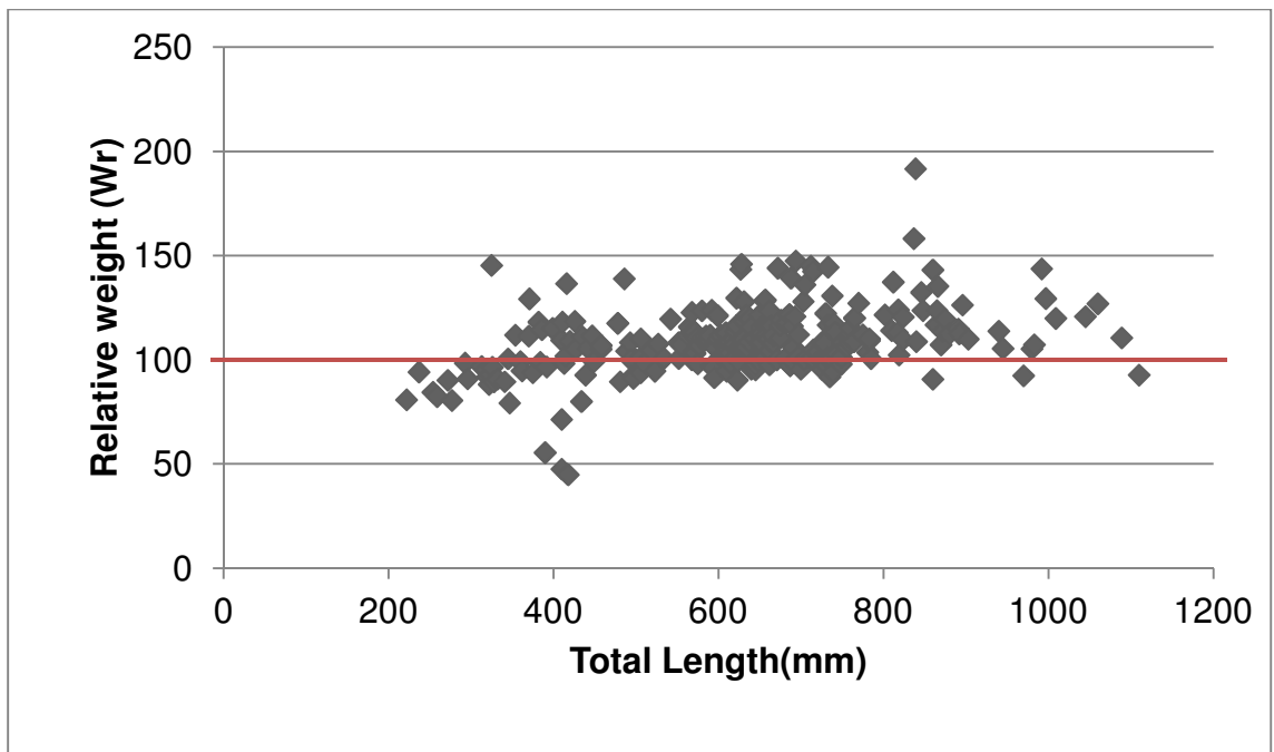
Figure 6. Relative weights for 298 northern pike in Box Canyon Reservoir collected in 2009 and 2010. Score of 100 is ideal for northern pike (Carlander 1969).
