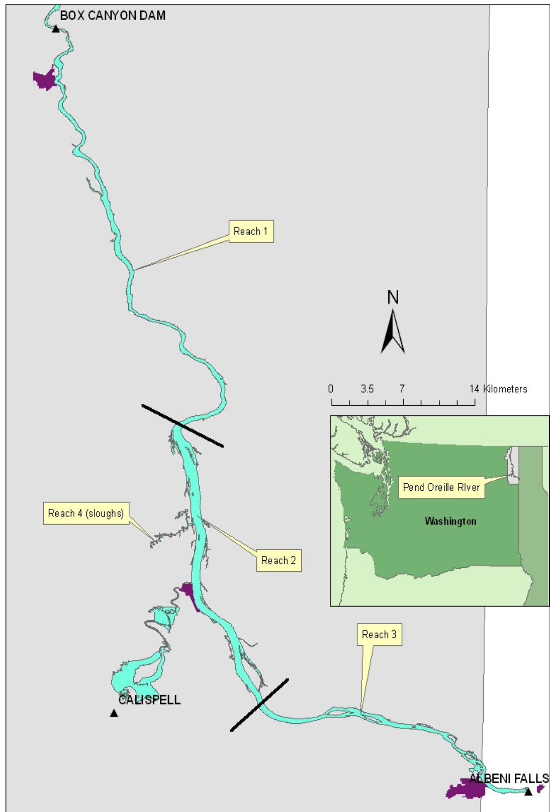
Figure 3. Locations of reaches and reach breaks for Box Canyon Reservoir used in this study.
