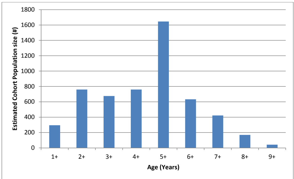
Figure 4. Estimated distribution of northern pike population by age class for Box Canyon Reservoir in 2010. Age 0 not shown because they were not fully recruited into the gear used.
