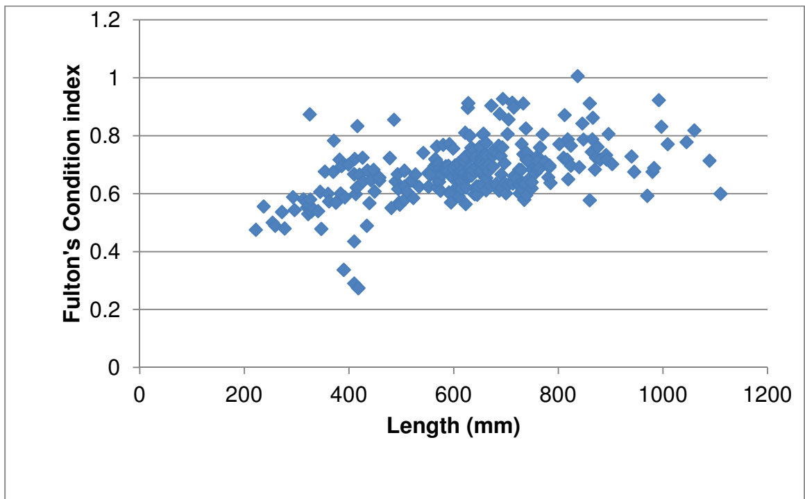
Figure 7. Fulton's condition index for 298 northern pike in Box Canyon Reservoir collected in 2009 and 2010. The average North American northern pike range from 0.47 to 0.69 (Carlander 1969).
