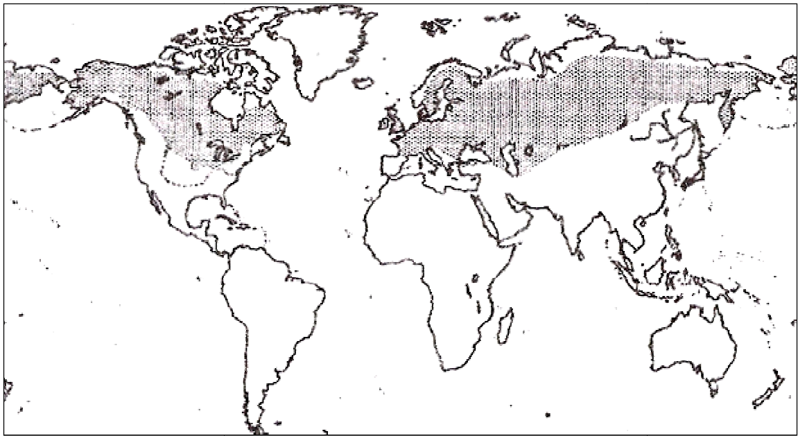
Figure 1. Geographical distribution of northern pike, limited to the cold temperate regions which are circumpolar in the Northern Hemisphere (Image courtesy of Ratt 1988).
