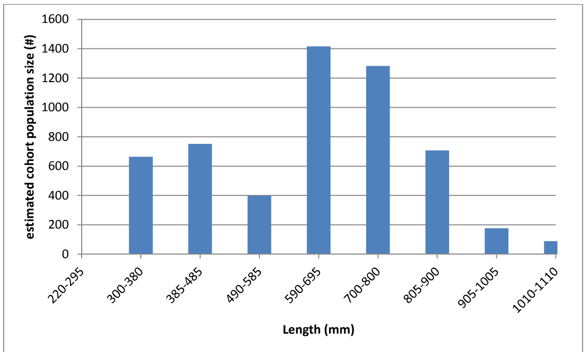
Figure 5. Estimated length distribution of northern pike population for Box Canyon Reservoir 2010. Northern pike less than 300 mm not represented because they were not fully recruited into the gear used.
